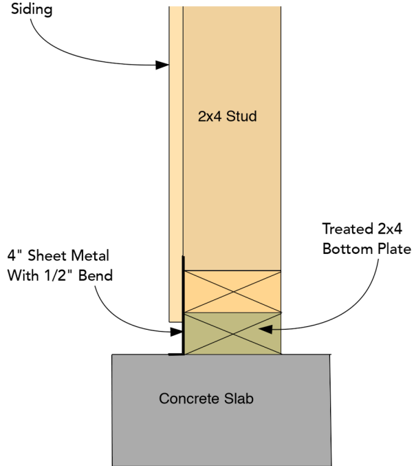
WALL BOTTOM FLASHING
