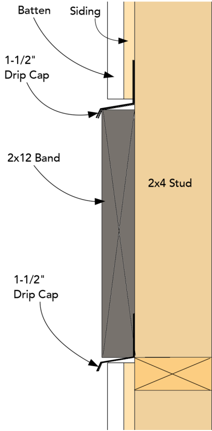
2x12 BAND FLASHING
