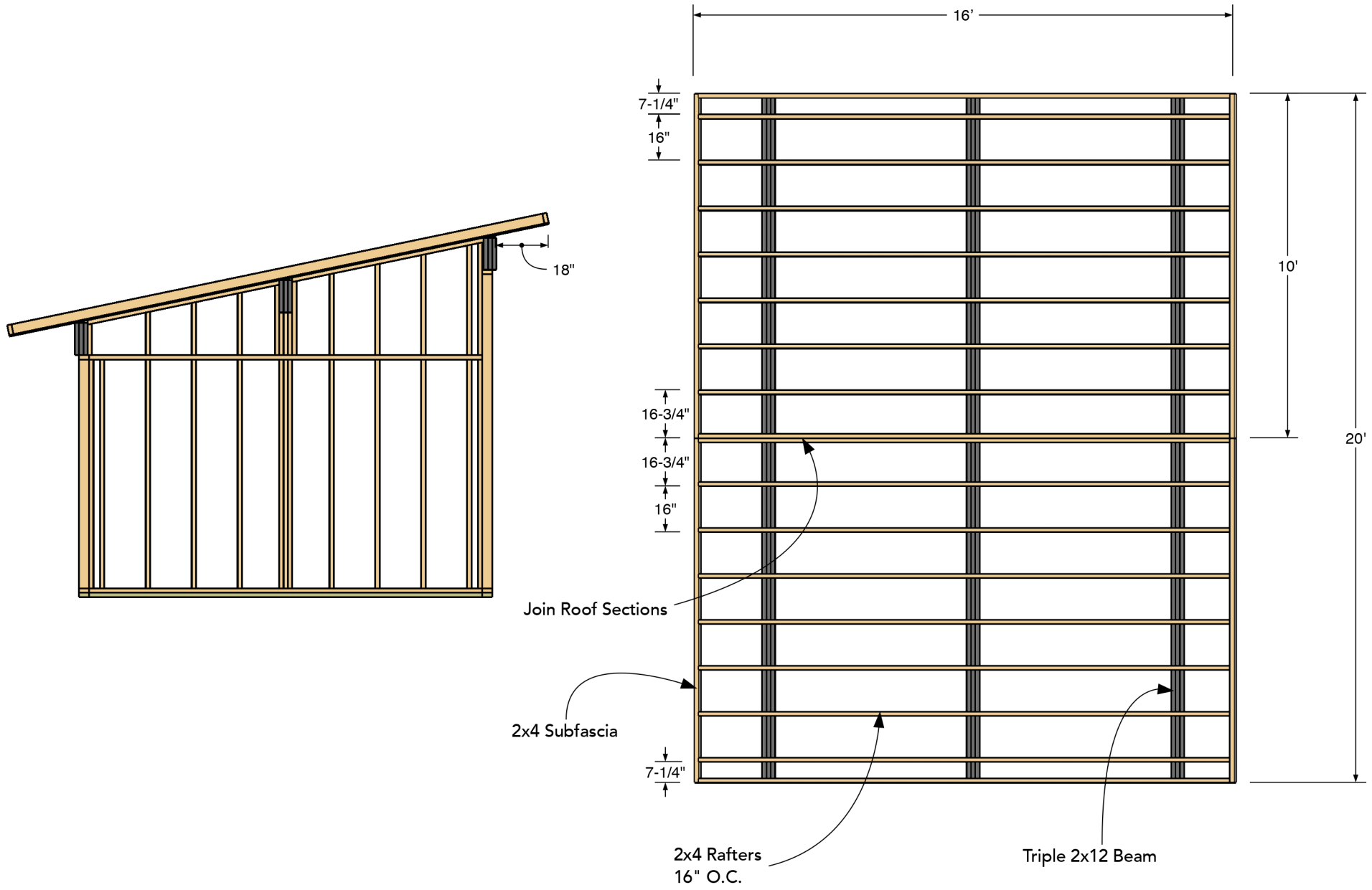
Figure G Roof Framing
