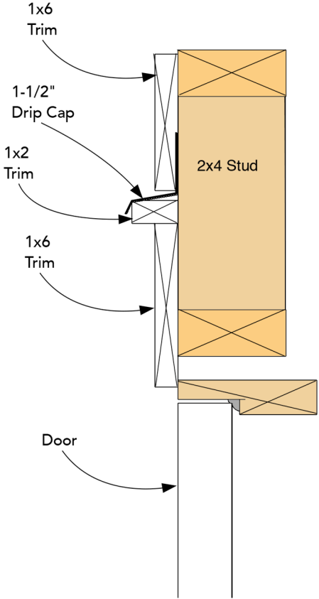
STORAGE DOOR FLASHING
