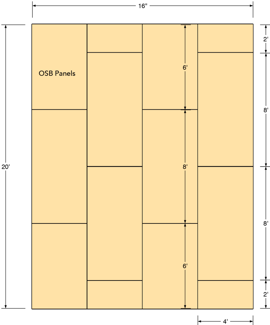
ROOF SHEATHING LAYOUT
