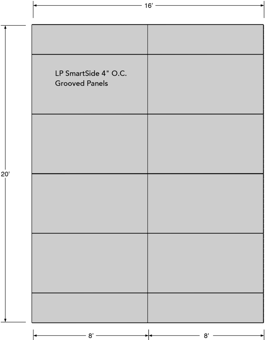
CEILING PANEL LAYOUT
