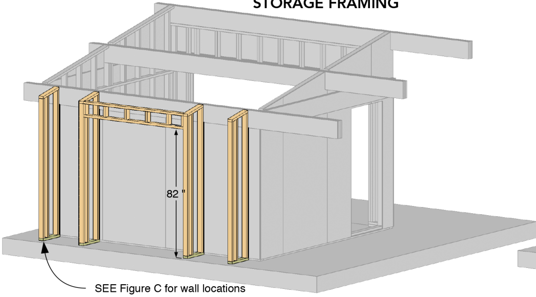
Figure M Storage Framing, Siding and Trim
