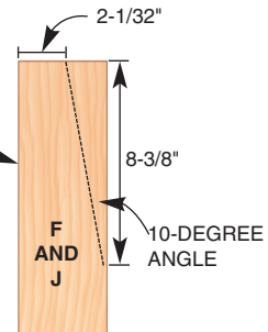
Figure B Top of Upright
