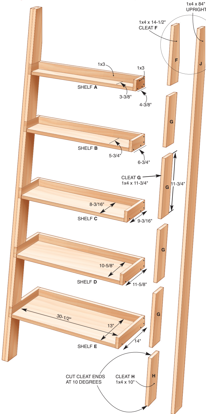
Figure A Modular Shelf Assembly
