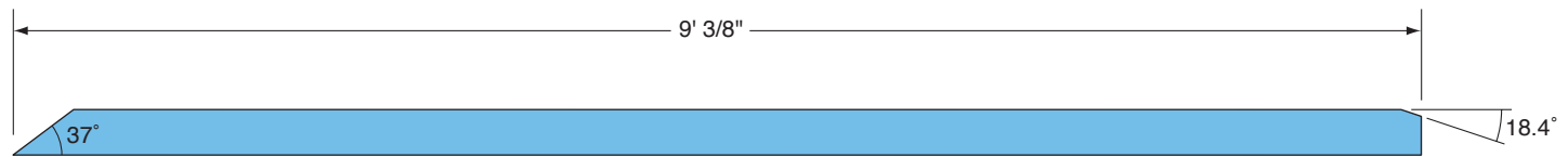
CROSS-TIE 6 (3 REQ'D)
