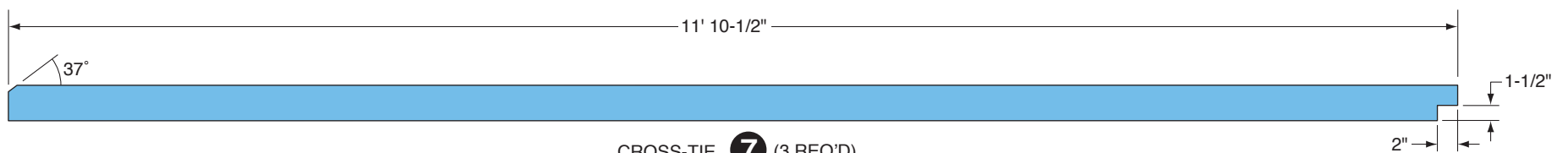
CROSS-TIE 7 (3 REQ'D)
